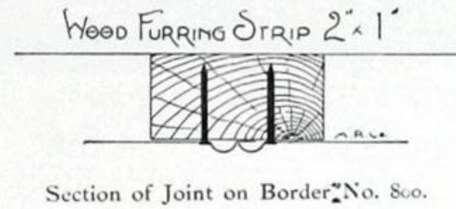
Section of Joint on Border No. 800.
